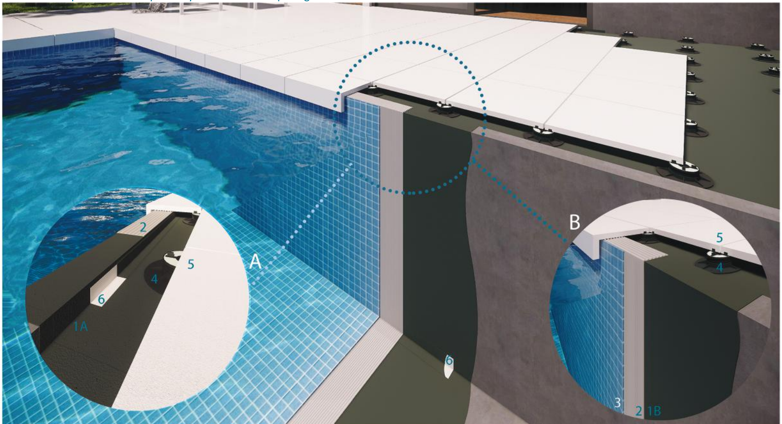
model of the pool with waterproof layers and ceramic paving
